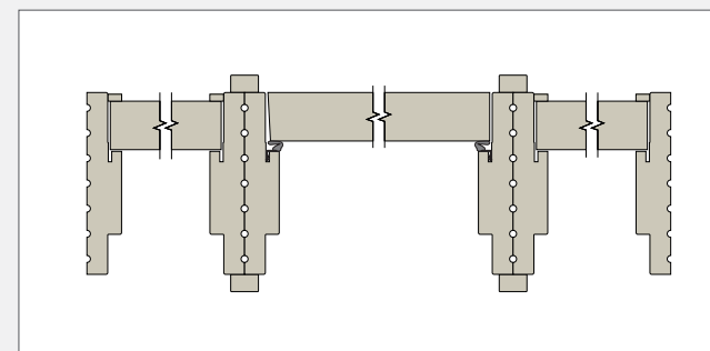
Double Rabbet Frame with Back-to-Back Mull Posts Accommodates screen door applications
