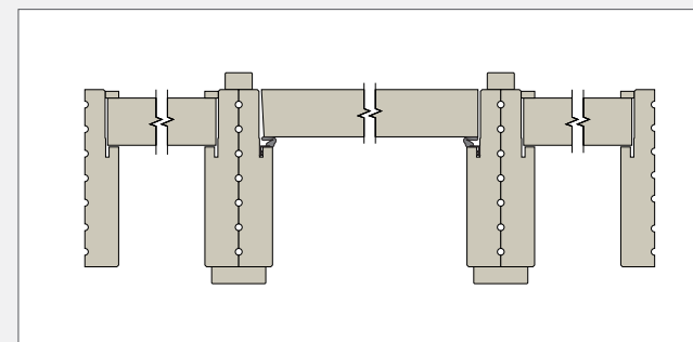
Single Rabbet Frame with Back-to-Back Mull Posts Default for all door applications
