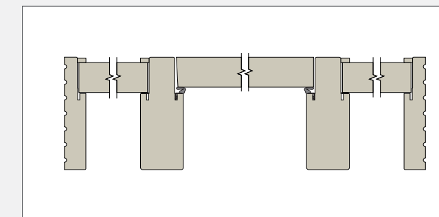
Single Rabbet Frame with 6-9/16" Uniframe Mull Posts
