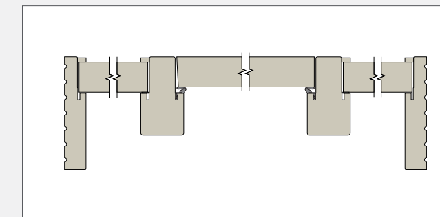
Single Rabbet Frame with 4-9/16" Uniframe Mull Posts
